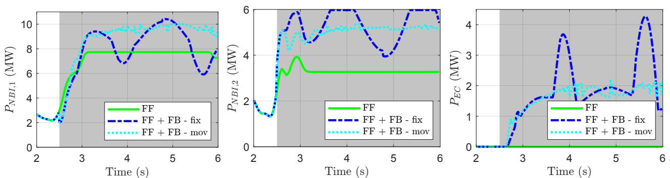
Fig. 3: Fixed and moving ECCD cases: Auxiliary powers - P_{NBI,1} (left), P_{NBI,2} (center), P_{EC} (right)
